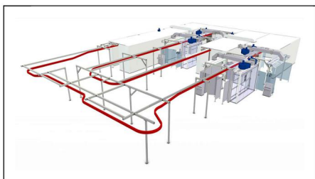
Overhead I-beam conveyors
